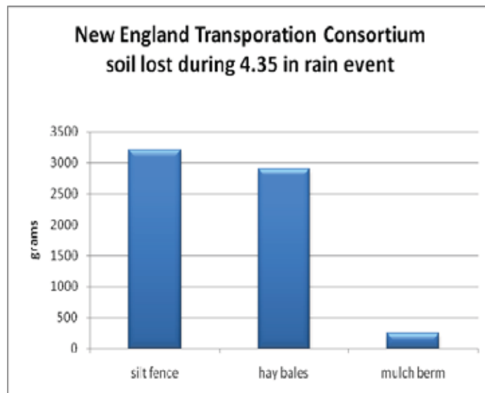
Figure 1. Sediment removal comparison (Source: Dumars et al, 2000)
